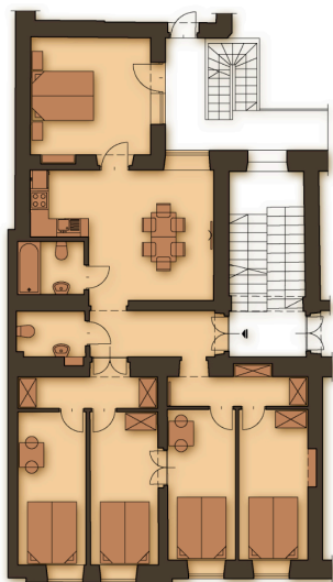
Apartment plan
