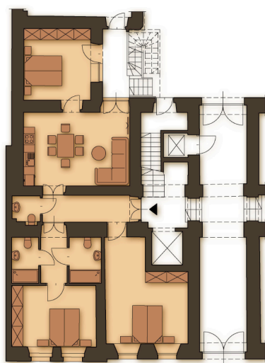
Apartment plan
