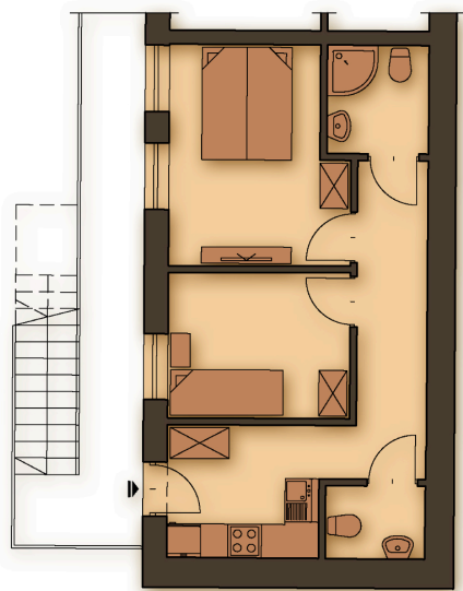
Apartment plan
